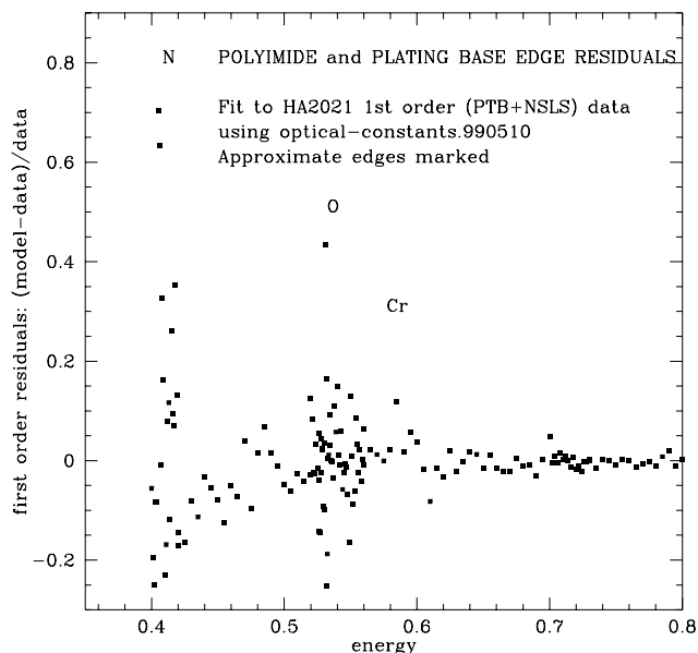
Figure 12. Residuals from the first order fit of grating HA2021, in the polyimide and plating base edge region. Although the residuals at the N and O edges are high, they are nevertheless significantly improved by the use of the new optical constants.
