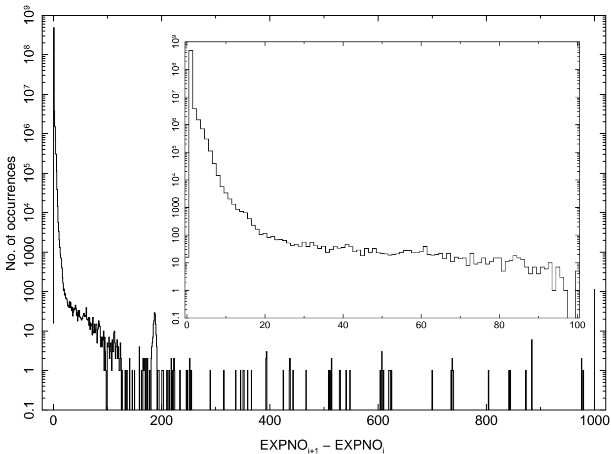
Figure 1: A histogram of the differences between consecutive frame numbers for 63,778 exposure-records files. A separate histogram was computed for each node of each file. The histogram in this figure is a sum of each of these histograms. If a difference is greater than 1000, then the difference is set to 1000. If a difference is less than 0, then the difference is set to 0. The inset histogram is a plot of the same data, except that it includes only the data in the range from 0 to 100. The histogram includes all frames, whether they are valid or not.
