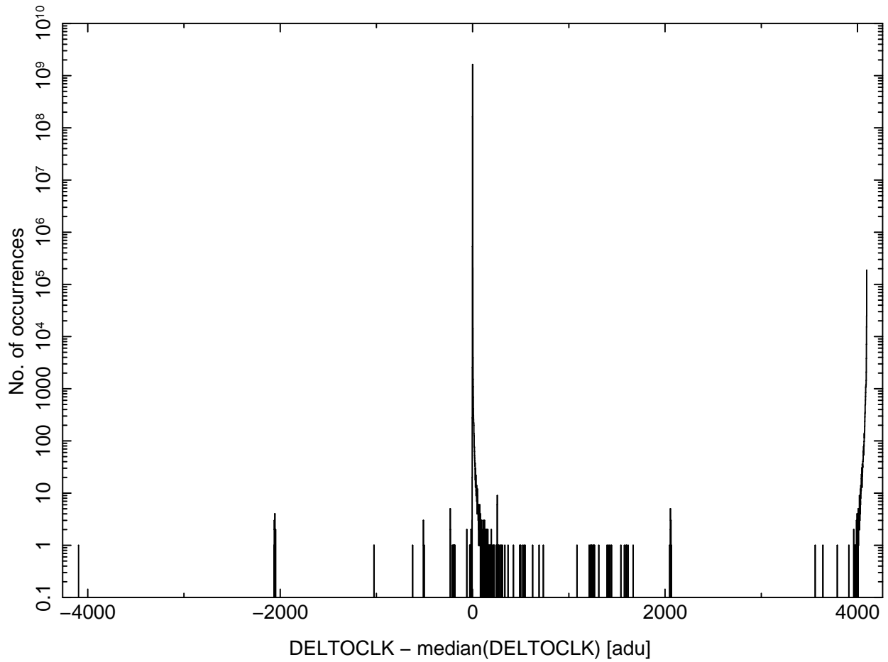
Figure 2: A histogram of the differences between the values of DELTOCLK and the values of the median DELTOCLK for 63,778 exposure-records files. A separate histogram was computed for each node of each file. The histogram in this figure is a sum of each of these histograms. The values of the median were computed using a numframes = 5 , maxframegap = ∞ , and minnumframes = 3 . If a value of DELTOCLK differs by more than 4096 adu from the corresponding median, then the difference is set to 4096 or -4096 as appropriate.
