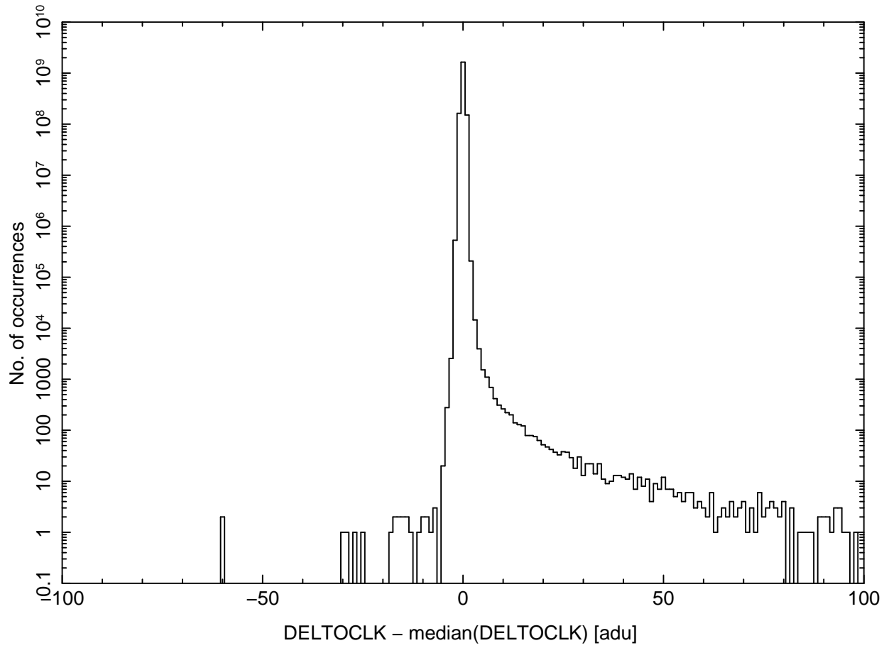
Figure 3: This figure is identical to Figure 2, except that it includes only the data in the range from -100 to 100 adu.
