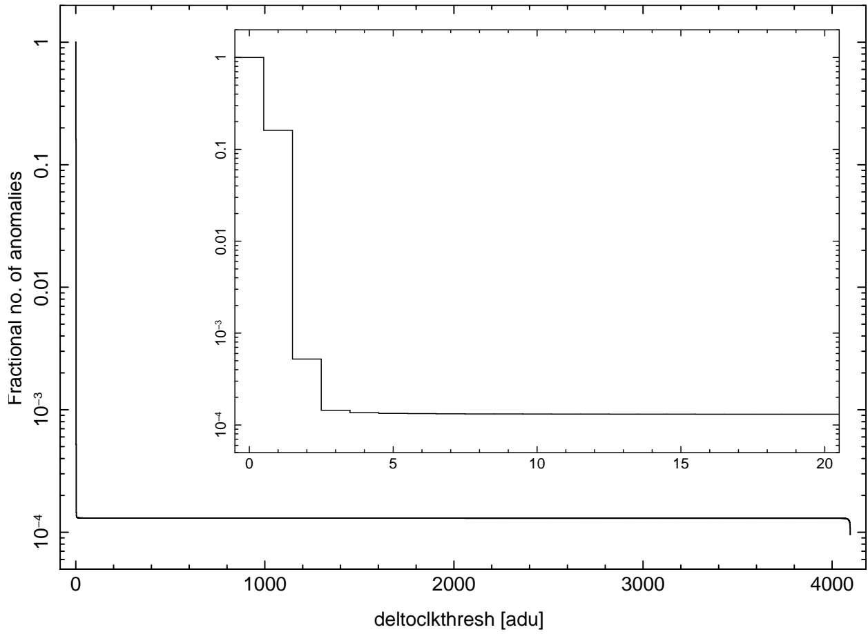
Figure 4: A plot of the fraction of the values of DELTOCLK that are identified as anomalous as a function of the parameter deltoclkthresh . This plot was produced using the data that is shown in Figure 2. The inset histogram is a plot of the same data, except that it includes only the data in the range from 0 to 20.
