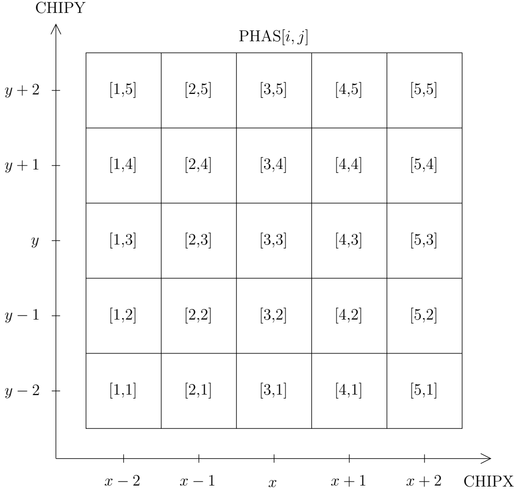
Figure 1: The relative CHIPX and CHIPY coordinates of the twenty five elements PHAS[ i, j ] of a 5 pixel \times 5 pixel event island with (CHIPX, CHIPY) = ( x, y ).
